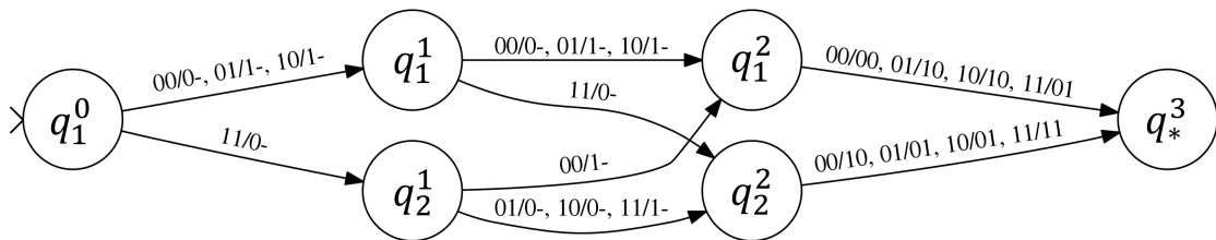
(a) FSM before state minimization.
