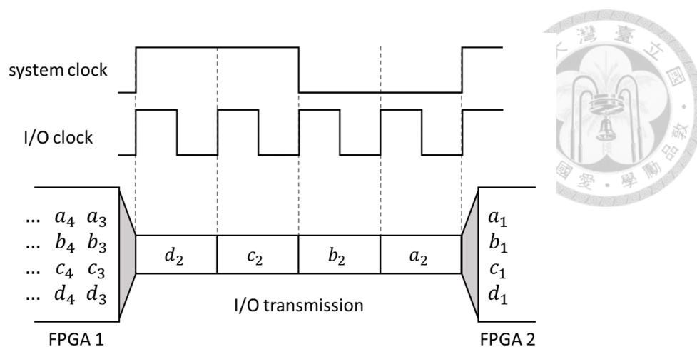
Figure 1.4: TDM I/O transmission with ratio 4.
