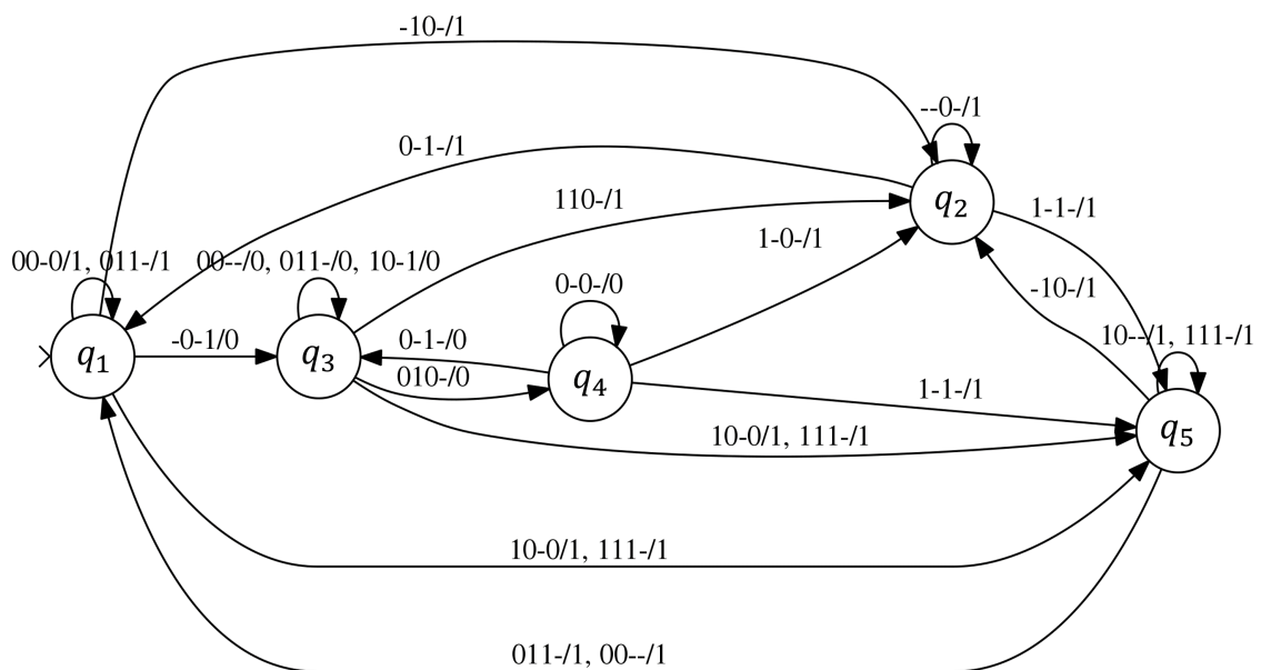
(c) FSM of original s27 circuit.
