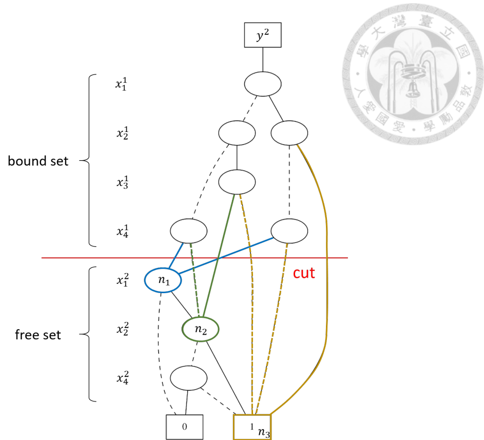
Figure 2.4: BDD-based functional decomposition.
