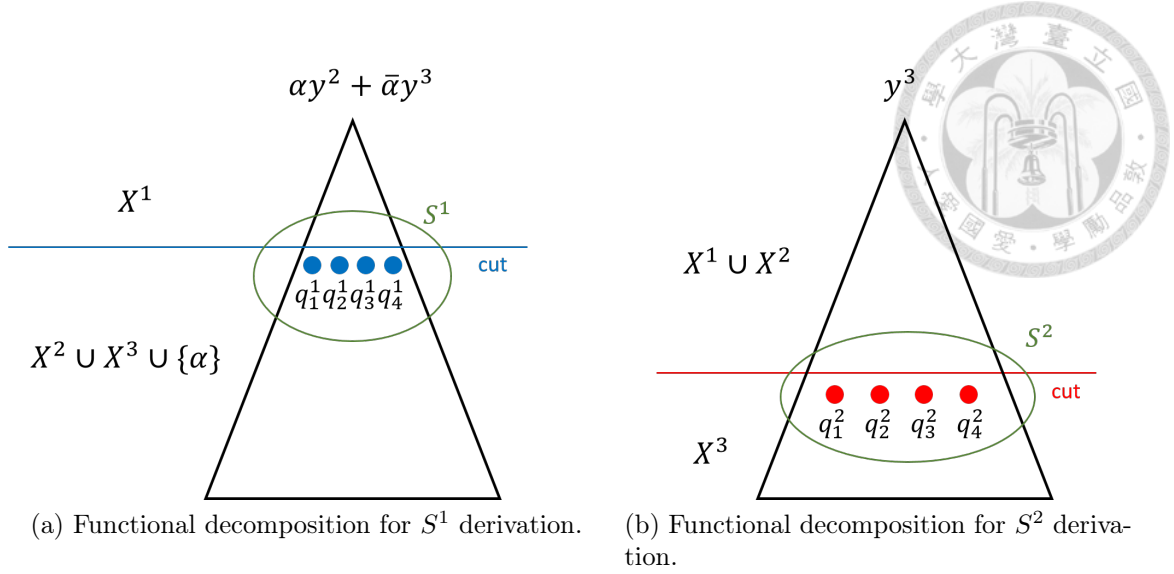
Figure 3.2: State identification.
