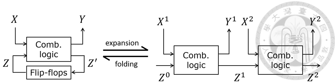
Figure 1.1: Time-frame expansion vs. folding.
