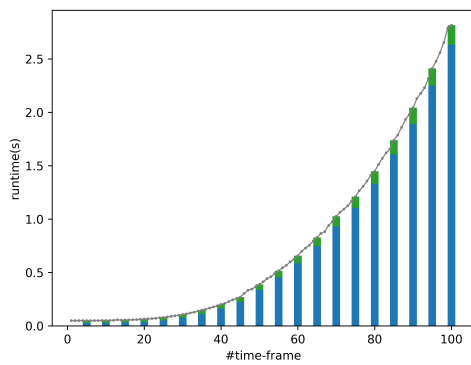
(c) s499
