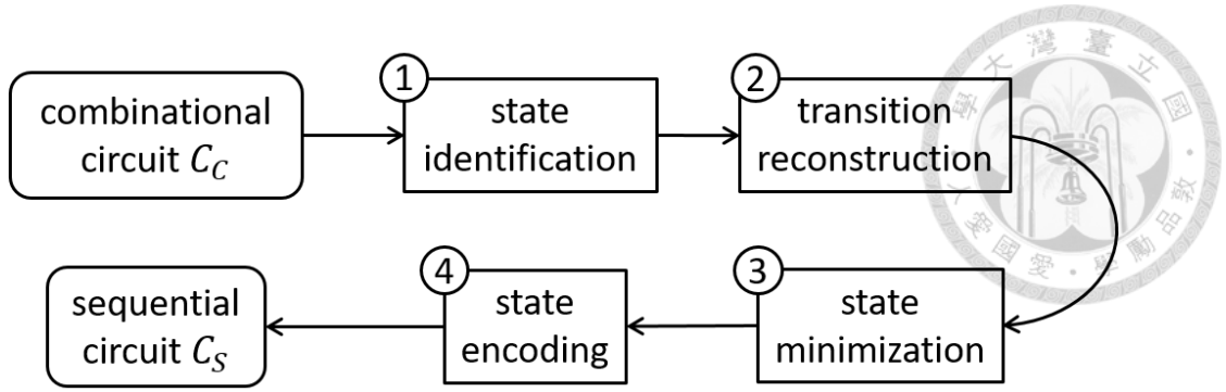
Figure 3.1: Computation flow of time-frame folding.
