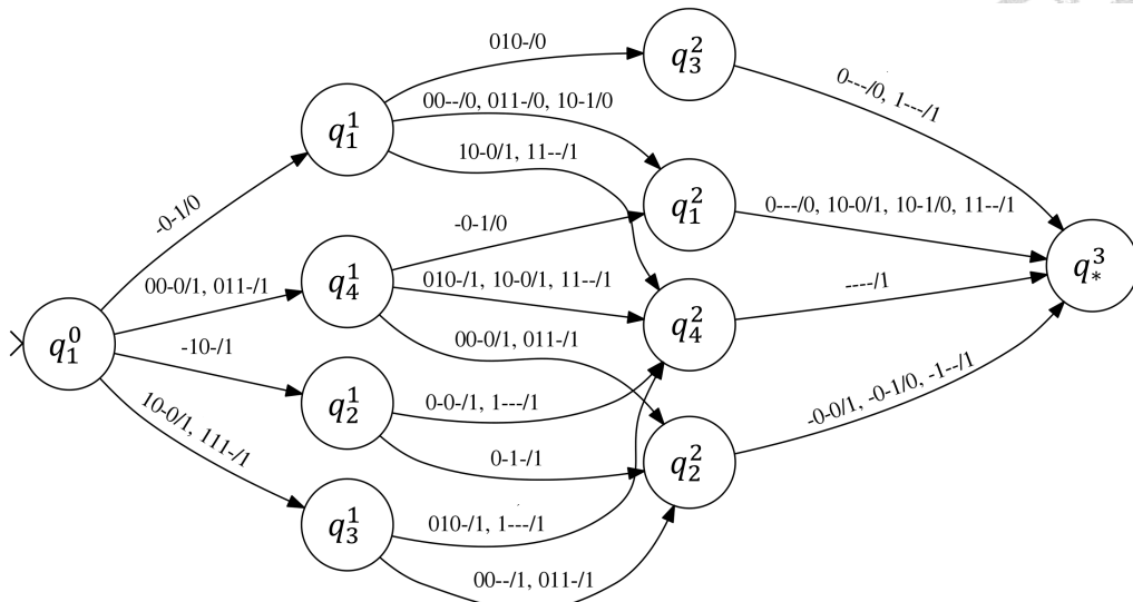
(a) FSM from folding 3 time-frames (before state minimization).
