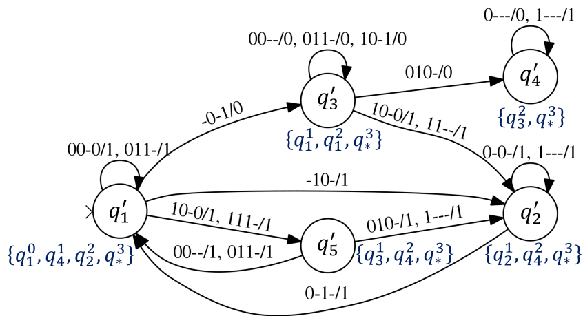
(b) FSM from folding 3 time-frames (after state minimization).
