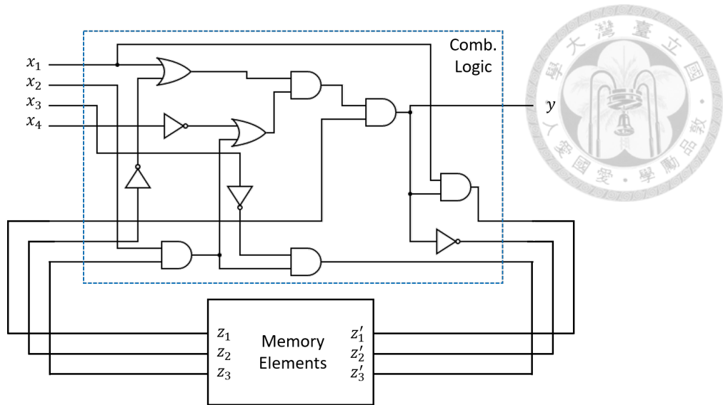
Figure 2.1: Sequential circuit s27.
