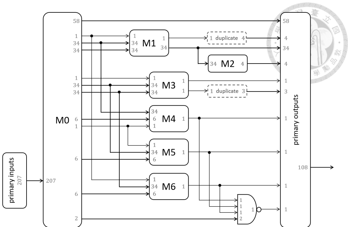
Figure 5.6: Hierarchical structure of C7552.
