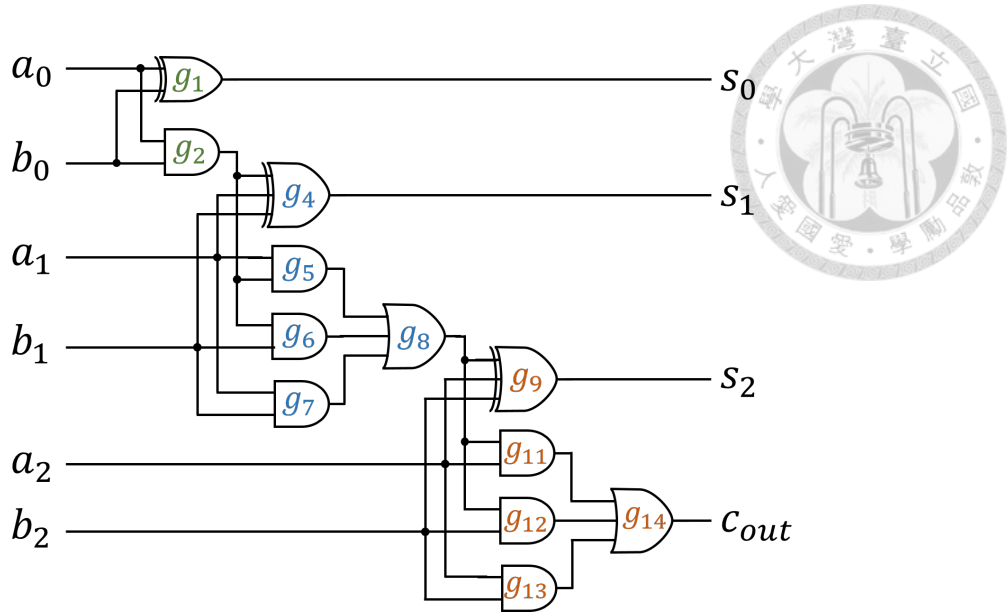
Figure 4.2: Example of 3-bit adder (3-adder) circuit under folding.
