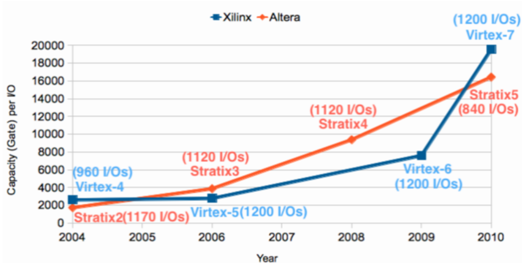
Figure 1.3: The ratio FPGA logic capacity over I/Os (retrieved from [32]).
