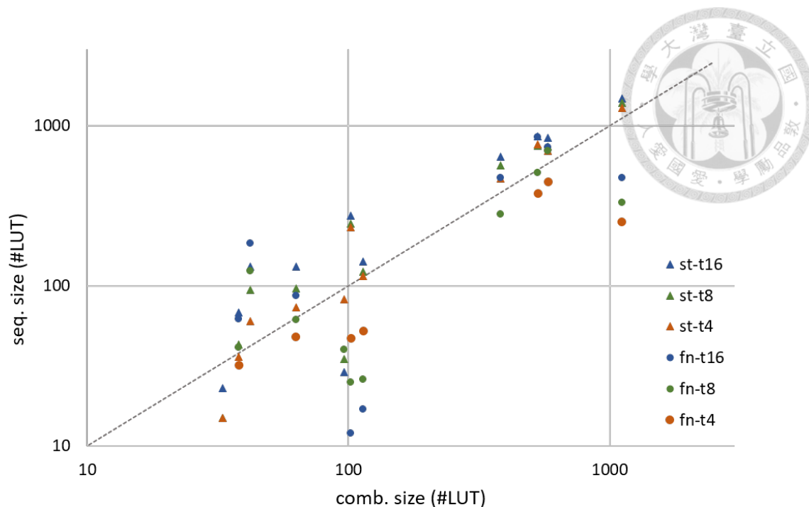
Figure 5.5: Circuit size comparison between structural and functional folding.
