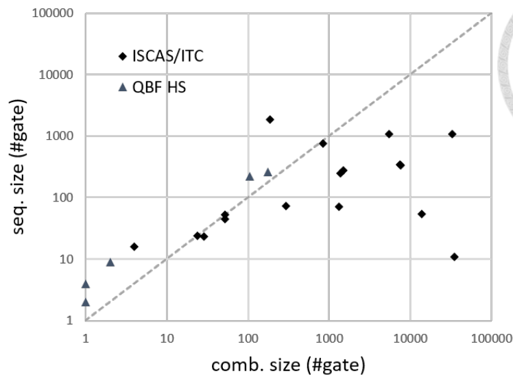
Figure 5.3: Circuit size after TFF.
