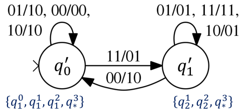
(b) FSM after state minimization.
