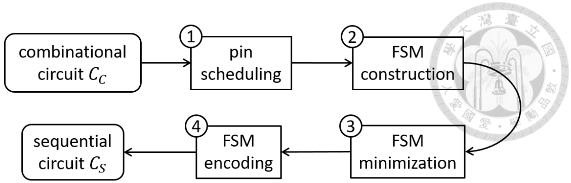
Figure 4.3: Computation flow of functional circuit folding.
