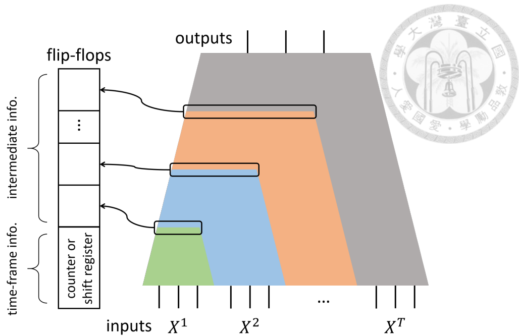
Figure 4.1: Illustration of structural circuit folding.
