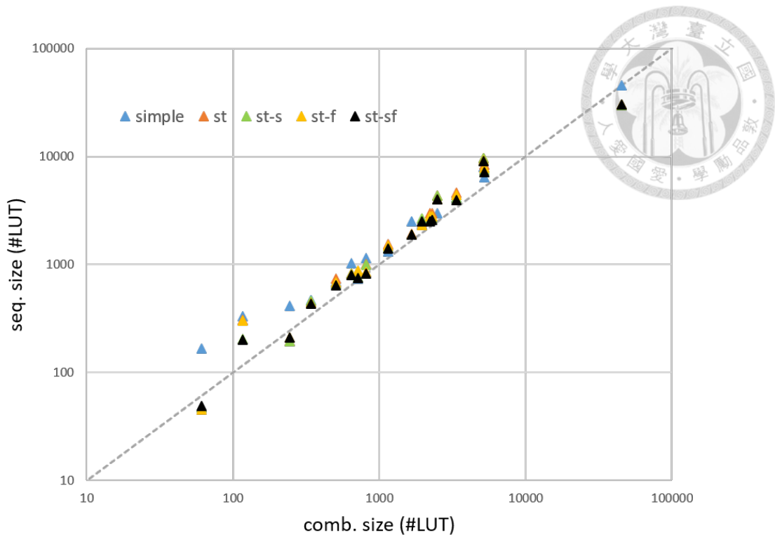
Figure 5.4: Circuit size after structural folding.
